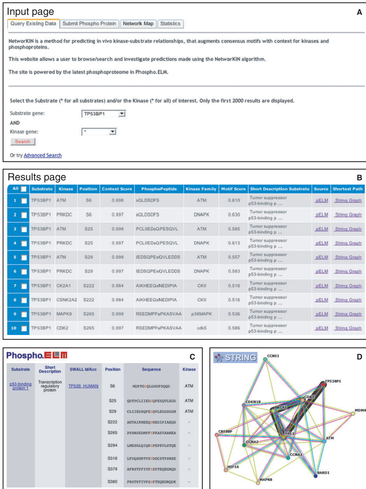
Figure 2. Using NetworKIN. A researcher is interested in the 53BP1 tumour suppressor. From the homepage of NetworKIN, this protein is chosen as the substrate protein to query the database for predictions relating any kinase to specific phosphorylation sites within 53BP1 (A). The system returns a total of 78 relations involving 12 different kinases that are predicted to phosphorylate 39 different sites, which are presented in a tabular view (B), (only the first 10 predictions are shown). These predictions can now be investigated in further detail by following either the links to the Phospho.ELM and PhosphoSite databases for curated knowledge related to the sites (C), or by following the links to the STRING network viewer to visualize the most probable path in the protein association network, which connects the kinase and the substrate (D).
