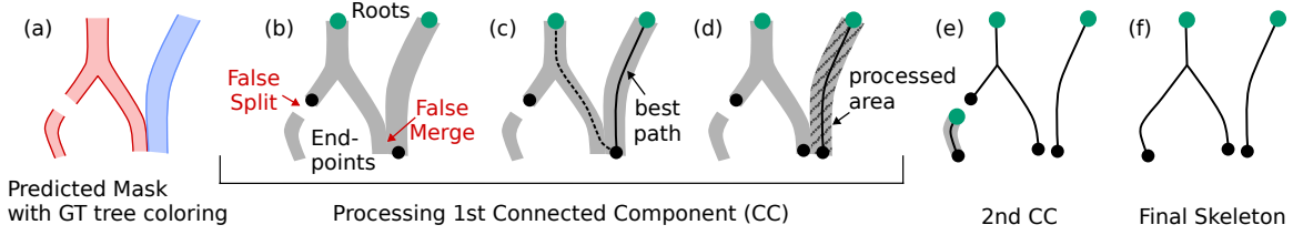
Figure 3: Addressing topological errors with the modified TEASAR algorithm.
