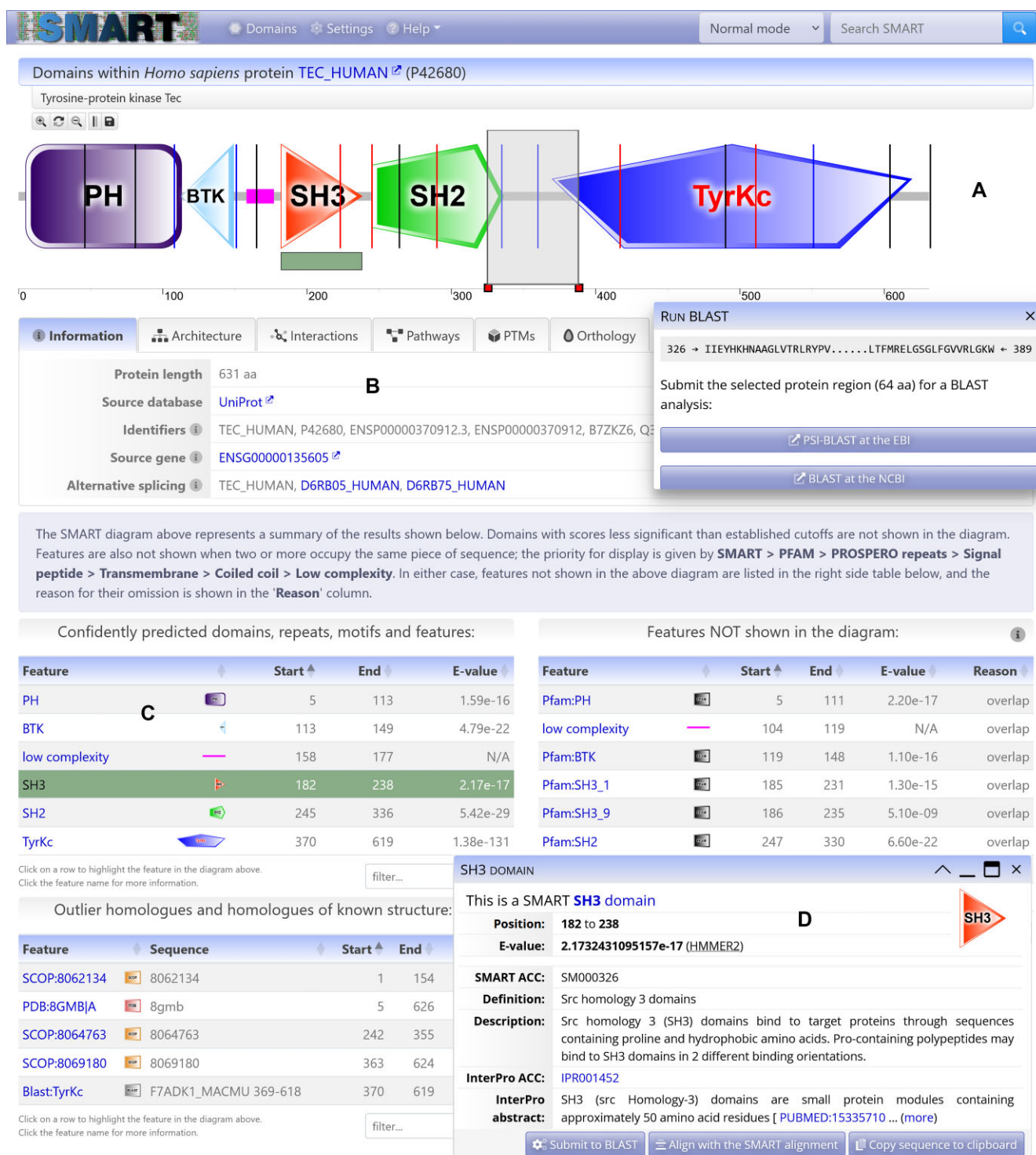
Figure 1. SMART annotation page for protein TEC_HUMAN . (A) Protein schematic representations are displayed using an interactive SVG (scalable vector graphics) applet. Schematics are zoomable without quality loss and can be saved as vector (SVG) images. Using the interactive scale, any protein region can be selected and submitted for further BLAST (Basic Local Alignment Search Tool) analysis. (B) Tabbed interface collects various sources of external information about the protein analyzed. (C) Data tables listing the domains and other features detected in the protein. Each table can be individually searched or sorted on any column. Selecting a feature will highlight it in the protein schematic, while scrolling the display to make it visible on screen. (D) Movable and resizable popup dialog displays the most important bits of information for any selected feature, with links to complete annotation.
