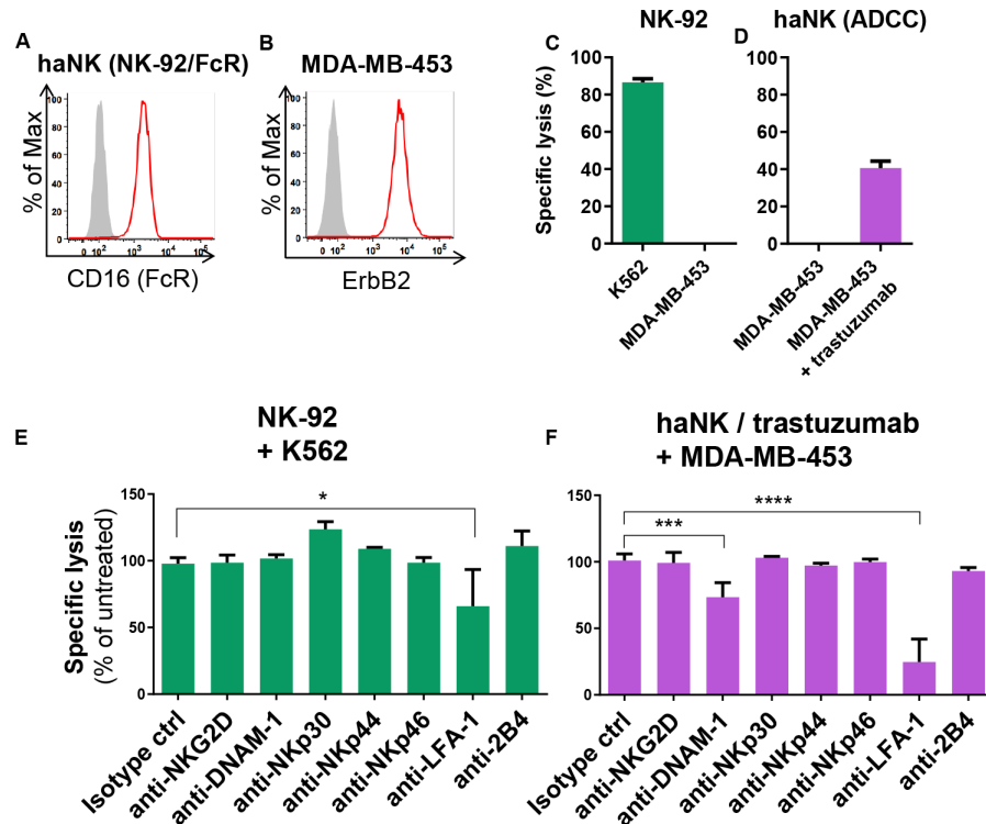
Figure 1 Blockade of LFA-1 alleviates natural cytotoxicity and ADCC of NK cells. (A, B) Histograms confirm FcγRIIIa (CD16) expression on haNK cells (A) and ErbB2 expression on MDA-MB-453 breast cancer cells (B). Filled gray areas indicate isotype controls. Representative data from at least three independent experiments are shown. (C, D) NK-92 (C) or haNK (D) cells were co-cultured with K562 or MDA-MB-453 cells at an effector to target ratio of 10:1 for 2 hours, and specific cytotoxicity was measured using a Europium-based cytotoxicity assay. Trastuzumab was added where indicated at a concentration of 2 μg/mL. Mean values from three independent experiments ± SEM are shown. (E, F) The indicated receptors on NK-92 (E) or haNK (F) cells were blocked with specific antibodies (20 μg/mL) for 60 min, followed by 2 hours co-culture with K562 or MDA-MB-453 cells. Isotype control IgG1 is shown (IgG2b was comparable). Trastuzumab (2 μg/mL) was added as indicated. Specific cytotoxicity was measured using a Europium-based cytotoxicity assay and is depicted as the percentage of cytotoxicity in the absence of blocking antibodies. Data were pooled from at least three independent experiments. Mean values ± SEM are shown. ADCC, antibody-dependent cell-mediated cytotoxicity; haNK, high-affinity FcγRIIIa-modified NK-92 cells; NK, natural killer.
