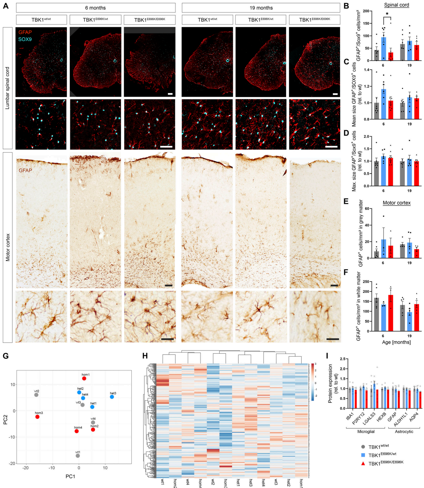
Figure S2. Analysis of astrocyte count and morphology in the lumbar spinal cord and motor cortex as well as proteomic analysis of glial markers in the lumbar spinal cord from TBK1^{E696K} knock-in and wt siblings. (A) Representative photomicrographs of LSC and motor cortex slices from 6- and 19-month-old TBK1^{E696K} knock-in and wt mice stained against the astrocytic markers GFAP and SOX9. Scale bars: 100 \mu\text{m} , 50 \mu\text{m} , 25 \mu\text{m} . (B-F) Quantification of the abundances, mean and maximal sizes of astrocytic cells in the spinal cord, and the gray and white matter of the motor cortex. Mean \pm SEM of n = 3-8 male mice per genotype from two independent experiments; two-way ANOVA with post hoc Tukey's multiple comparisons test; *P < 0.05 in B. (G and H) Principal component and heatmap hierarchical clustering analysis of glial proteins in LSC lysates from 19-month-old mice does not show separation of the three genotypes. N = 4 male mice per genotype. (I) Expression of selected glial markers in LSC at 19 mo. Mean \pm SEM of n = 6 male mice per genotype; two-way ANOVA with post hoc Tukey's multiple comparisons test.
