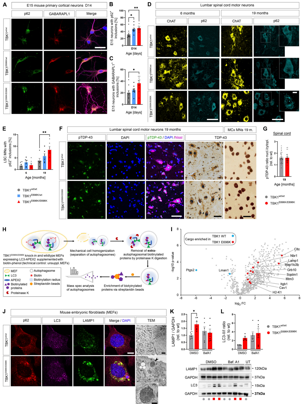
Figure 4. TBK1 E696K/E696K knock-in impairs autophagy in cell models and mice. (A) Representative photomicrographs of TBK1 E696K/E696K knock-in and wild primary cortical neurons stained against p62 and GABARAPL1. Scale bar: 10 \mu m. (B and C) Quantification of large p62 + and GABARAPL1 + inclusions in primary
