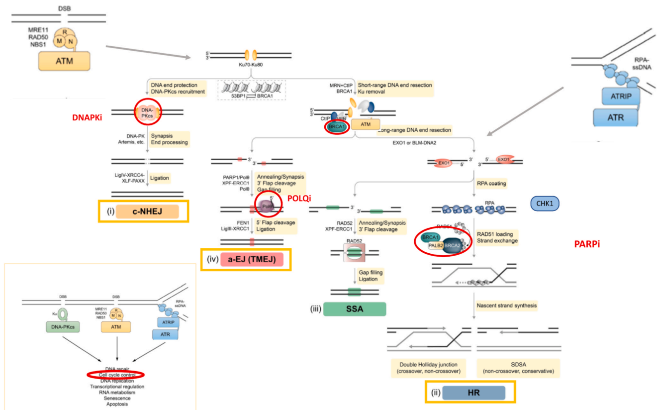
Fig. 1. DNA damage response pathway. a-EJ, alternative end joining; c-NHEJ, classical non-homologous end joining; HR, homologous recombination; SSA, single-strand annealing.
