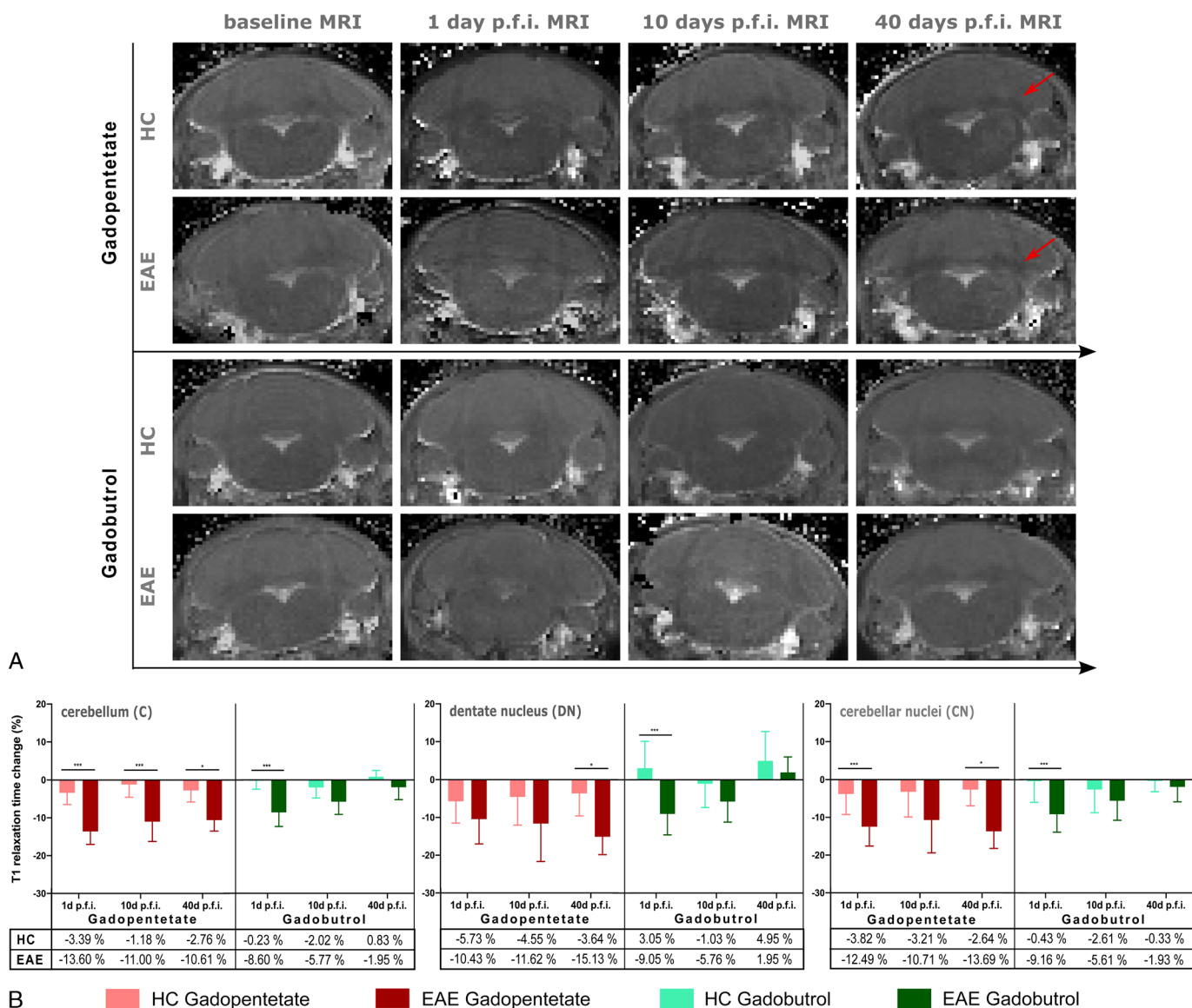
FIGURE 3. 7 T MRI relaxometry in vivo. A, Representative longitudinal MRI scans (T1 map RARE-VTR sequence) of animals sacrificed 40 days pfi of GBCAs. Relaxometry revealed decreasing T1 relaxation times within the CN (red arrow) toward day 40 pfi of gadopentetate in EAE and HC animals. Gadobutrol-treated animals did not show prominent qualitative T1 shortening within the CN. B, T1 relaxation time change (%) differences between EAE and HC animals within the C, DN, and CN for both tested GBCAs. Mann-Whitney tests were computed for EAE versus HC after gadopentetate or gadobutrol treatment and the Bonferroni correction was applied for multiple testing over 3 consecutive time points. Data are displayed as mean \pm SD.
