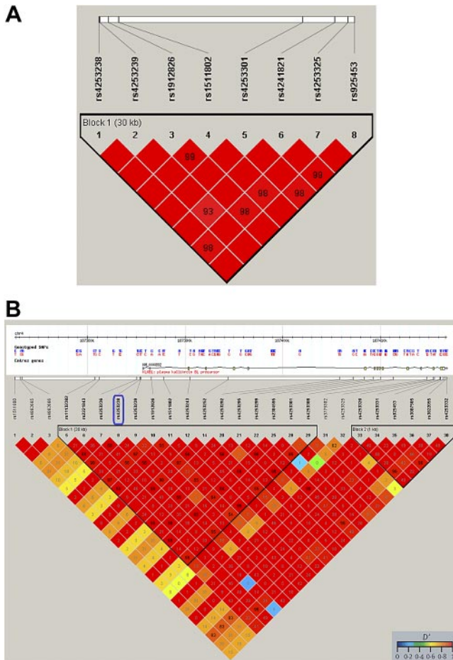
Figure 3. SNP rs4253238 is in LD with other KLKB1 SNPs. A) LD plot of the GWAS identified SNP rs4253238 identifies a block of LD between this SNP and other SNPs present in the KLKB1 gene, in the control/asthma data set ( n=584 ). B) LD plot generated with Haploview, utilizing HapMap data selected for the CEU (Utah residents with northern and western European ancestry) population, confirms the presence of a block of LD for SNP rs4253238 with SNPs in the 5' region of the KLKB1 gene. Numbers identify the R^2 values up to a maximum of 100. The color scheme denotes the level of LD as defined by D' . Similar plots identify no LD with regions downstream of rs4253238 (data not shown).
