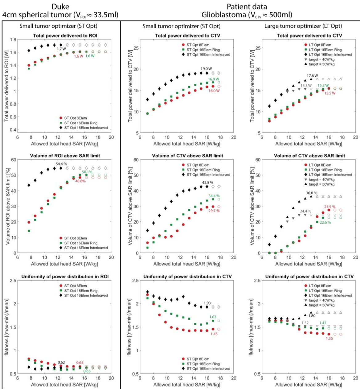
Figure 4: Quantitative evaluation of optimizer performance for Duke with the 4cm tumor (left) and the patient voxel model (middle and right) comparing the total delivered power (top), the fraction of the target region with a SAR higher than the given limit for the OAR (40W/kg) and the non-uniformity of the power distribution (bottom).
