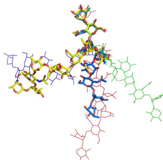
Glyc_1stRU_restricted
