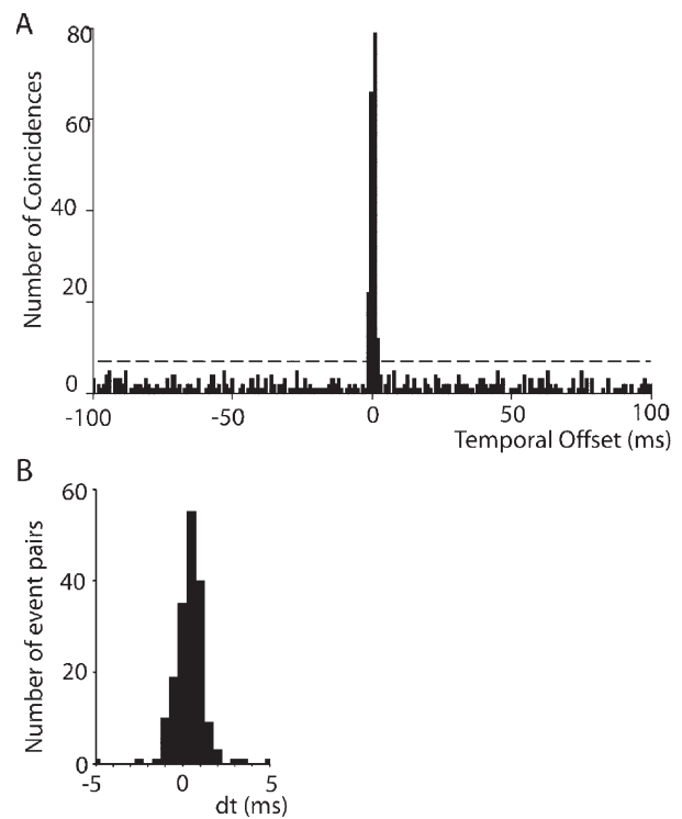
Figure S3. Cross correlation histogram of the coincident events from the experiment shown in Fig. 6. (A) Cross correlation histogram of events in principal neuron and NG2 glia. The dashed line indicates the chance level. Event traces from NG2 glia and neuron were binned with a temporal resolution of 1 ms and then cross-correlated. The sharp peak around zero disappears as soon as the traces are shifted more than 2 ms in each direction. No other time relation than \pm 2 ms is visible. (B) Magnification of the peak of the time-difference histogram of events in NG2 glia related to neurons in Fig. 6 E. The time difference between events in the two cells is plotted as a histogram. The bin width was 0.5 ms. Note the delay of the peak of +0.5 ms.
