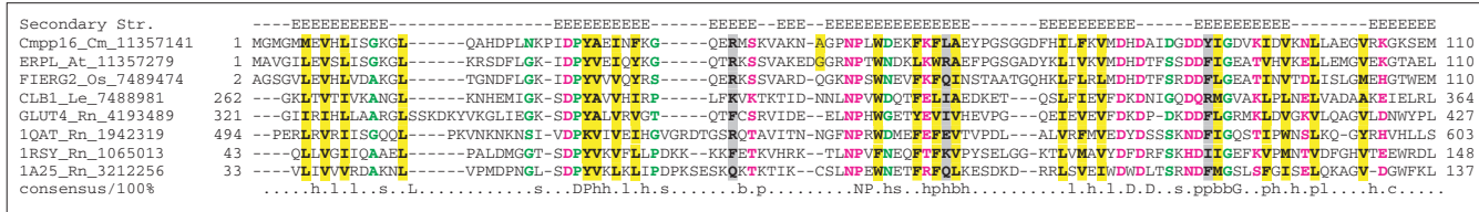
Figure 6 Multiple alignment of a selection of C2 domains including the alleged 'paralog' of plant virus movement proteins, Cmp16. The scheme for displaying multiple alignments is as described in the legend to Figure 1. Residues are colored at 100% consensus. A consensus secondary structure was derived from known structures of the C2 domains in phospholipase C- \delta 1 (IQAT), synaptotagmin (IRSY), and protein kinase C (IA25). At: A. thaliana , Cm: Cucurbita maxima , Le: Lycopersicon esculentum , Os: Oryza sativa , Rn: R. norvegicus .
