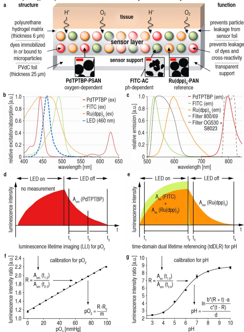
Figure 1: Dual 2D luminescence imaging of \text{pO}_2 and \text{pH}_e in vivo. (A) Sensor foil scheme: Oxygen-dependent palladium(II)-meso-tetraphenyltetrazeporphyrin incorporated in oxygen-permeable poly(styrene-co-acrylonitrile) particles (Pd-TPTBP-PSAN), pH-sensitive fluorescein-isothiocyanate bound to aminocellulose particles (FITC-AC), and the pH-independent reference dye ruthenium(II)-tris(4,7-diphenyl-1,10-phenanthroline) in oxygen-impermeable polyacrylonitrile particles (Ru(dpp) 3 -PAN). Microparticles were embedded in a polyurethane hydrogel matrix on poly(vinylidene-chloride) (PVdC) foils. Dye leakage was prevented by binding the dyes to or incorporating them into microparticles. By embedding the particles in hydrogel, leakage of particles from the sensor was also prevented. The insets show transmission electron-microscopic (TEM) pictures of the sensor particles (bars are: left and right image 0.5 \mu\text{m} , middle image 2 \mu\text{m} ). (B,C) Excitation (ex) (460 nm light emitting diode = LED) and emission (em) spectra of the sensor particles. Luminescence signals were optically filtered for \text{pO}_2 (800/60 filter) and pH (OG530 + S8023 filters) visualization. (D,E) Detection schemes for \text{pO}_2 and pH. Luminescence lifetime imaging (LLI) (D) was used for \text{pO}_2 -imaging. Luminescence intensities during emission were integrated in two separate time-frames, and a ratio (R) of these data gives a referenced signal for \text{pO}_2 . Time-domain dual lifetime referencing (tdDLR) (E) was used for pH-imaging. The combined signal intensities of pH-dependent FITC and pH-independent Ru(dpp) 3 were integrated in a time-gate during excitation, and only the long-lasting reference signal of Ru(dpp) 3 was detected in a time-gate during emission. The ratio (R) of these data gave a referenced signal for pH. (F,G) Calibration curves for \text{pO}_2 and pH. Solving the linear fit for \text{pO}_2 and the sigmoidal fit for pH enabled \text{pO}_2/\text{pH}_e -calculations for each pixel. Measured luminescence intensity ratios (R) obtained for each pixel were inserted in the respective equations to give referenced \text{pO}_2/\text{pH}_e -values, which displayed as pseudocolor maps to show the spatial distribution of these parameters.
