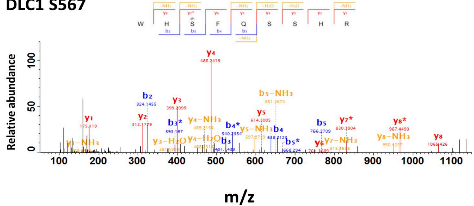
Figure S4. DLC1, DLC2, and DLC3 are AKT substrates. (A) In vitro AKT kinase assay. (A, top) IP DLC1-WT was strongly phosphorylated by recombinant AKT kinase (lane 2), as detected with 32 P autoradiography. GFP control gave no phosphorylation signal (lane 1). DLC2 (lane 3) and DLC3 (lane 4) were also phosphorylated, but weakly compared with DLC1. (A, bottom) Expression of GFP vector and GFP-tagged DLC constructs. (B) DLC1 phosphopeptides identified by mass spectrometry. Annotated tandem mass spectrometry spectra are shown for the three phosphopeptides containing phosphorylated S298, S329, and S567. b-Type fragments are shown in blue and y-type fragments in red. Water- and ammonia-loss peaks are shown in yellow, and neutral phosphate losses are indicated with asterisks. The fragment ions observed allow full localization of the phosphorylation sites on the serine residues noted in each peptide. Spectra were annotated using the Viewer software of the MaxQuant 1.3.0.5 software package.
