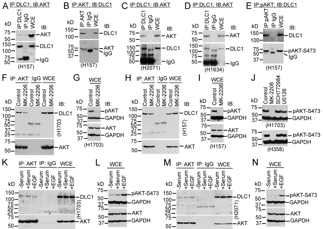
Figure S3. DLC1 and AKT forms a protein complex in human cell lines, and complex formation does not require enzymatic activity of AKT. (A) Endogenous protein complex between DLC1 and AKT. Lysates from H157 cells were IP with DLC1 or mock IgG antibodies followed by IB with AKT (top) or DLC1 (bottom) antibodies. WCE, whole cell extract. (B) The endogenous protein complex between DLC1 and AKT was confirmed by reciprocal coIP. (C and D) Experimental conditions and data display were similar to A, but for nontransformed lines H2071 (C) and H1634 (D). (E) Some AKTs that are associated with DLC1 are enzymatically active. Endogenous protein complex between DLC1 and kinase-active AKT (pAKT-S473) in H157 cells. Lysates were IP with pAKT-S473 antibody followed by IB with DLC1 (top) or pAKT-S473 (bottom) antibodies. (F) Complex formation between DLC1 and AKT did not require AKT enzymatic activity. The experimental conditions were similar to B, except that the protein complex between DLC1 and AKT was analyzed in the absence or presence of MK-2206 in H1703 cells. (G) MK-2206 treatment inhibited AKT activity (measured by pAKT-S473) in H1703 cells. (H) The experimental conditions and data display were similar to F, but for H157 cells. (I) MK-2206 treatment inhibited AKT activity in H157 cells. (J) MK-2206 is a specific AKT inhibitor because AKT activity (measured by pAKT-S473) was inhibited by MK-2206 in both H1703 and H358 lines but not by inhibitors of ERK (SCH772984) or MEK (U0126). (K–N) Stimulation of AKT by EGF treatment did not increase the AKT/DLC1 protein complex in H1703 (K) and H2071 (M) cell lines. EGF stimulated AKT activity, but not total AKT, in H1703 (L) and H2071 (N) lines. GAPDH was used as a loading control.
