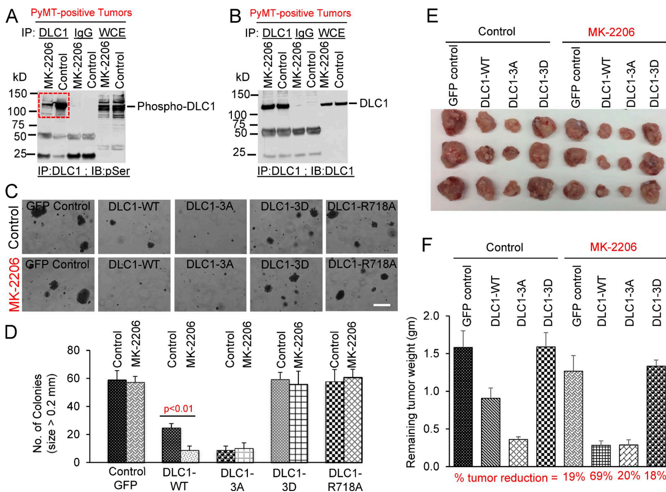
Figure S6. AKT inhibition has greater antitumor activity in DLC1-positive tumors. (A and B) Lysates from MMTV PyMT-positive tumors treated with or without MK-2206 were IP with DLC1 antibody followed by IB with (pSer) phospho-AKT substrate-specific (A) or DLC1 (B) antibodies. WCE, whole cell extract. MK-2206 treatment reduced serine phosphorylation (pSer) of DLC1 (A; compare lanes 1 and 2) without changing the DLC1 expression (B; compare lanes 1 and 2). (C) Anchorage-independent growth of H358 cells stably transfected with DLC1 mutant in the absence or in the presence of MK-2206. MK-2206 treatment inhibited growth and colony formation in soft agar of DLC1-WT transfected cells. However, MK-2206 treatment did not influence the anchorage-independent growth or the number of soft agar colonies of GFP control, DLC1-3A, DLC1-3D, or GAP-dead DLC1-R718A transfected cells. Bar, 2 mm. (D) Quantification of agar colonies (>0.4 mm) in the indicated groups from three independent experiments. Parametric two-tailed t tests were performed for statistical analysis. MK-2206 treatment induced a significant decrease ( P < 0.01 ) in soft agar colonies in DLC1-WT. However, MK-2206 treatment did not influence the soft agar growth of GFP, DLC1-3A, DLC1-3D, or DLC1-R718A transfected cells. Error bars in the graph indicate the SD. (E) Mice with tumors were treated with MK-2206 (50 mg/kg for 5 d) 8 wk after injecting the stable transfectants. Photographs of xenograft tumors from mice after treatment for 5 d with MK-2206. (F) Graph shows tumor weight (in grams) means \pm SD for each group in the presence or absence of MK-2206 treatment. The numbers below the graph represent the percent reduction in tumor weight by MK-2206 treatment compared with respective untreated group.
