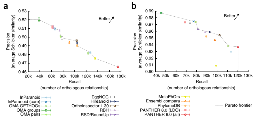
Figure 4 | Benchmarks of functional similarity between inferred orthologous gene pairs. Two different types of functional annotations are used: (a) experimentally supported GO annotations and (b) Enzyme Commission (EC) numbers. Error bars indicate 95% confidence intervals.
