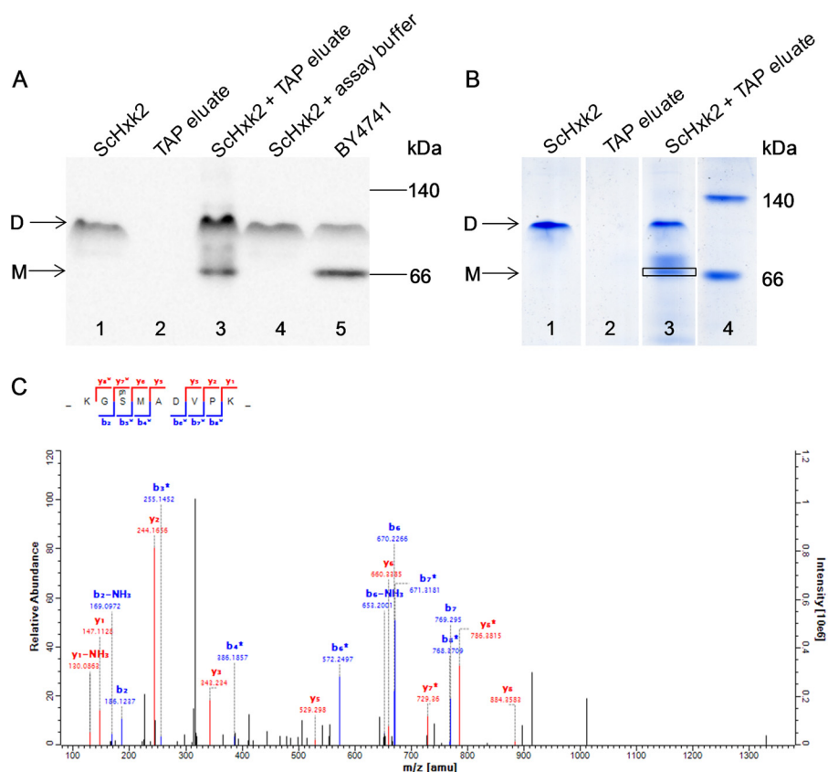
FIGURE 3. ScHxk2 in vitro phosphorylation with TAP-enriched Ymr291w protein kinase. A , immunodetection. Purified unphosphorylated ScHxk2 was incubated for 2 h with TAP eluate in 30 mM Tris-HCl buffer containing 5 mM ATP and 20 mM MgCl 2 at pH 7.4 and 30 °C ( lane 3 ). The unphosphorylated hexokinase ( lanes 1 and 4 ) and TAP eluate ( lane 2 ) were included as negative controls. BY4741 protein extract ( lane 5 ) was analyzed as a positive control to indicate the positions of the ScHxk2 monomer and dimer in the gel. Samples containing 25 ng of purified ScHxk2 ( lanes 1, 3, and 4 ), 10 ng of TAP eluate ( lanes 2 and 3 ), and 10 μg of BY4741 protein extract ( lane 5 ) were applied. For cell disruption, electrophoresis, and immunodetection, see the legend to Fig. 1. B , sample preparation for mass spectrometric analysis of Ymr291w-dependent ScHxk2 in vitro phosphorylation. The experiment described in A was modified by increasing the amounts of ScHxk2 (5 μg; lanes 1 and 3 ) and TAP eluate (0.2 μg; lanes 2 and 3 ) followed by protein staining with colloidal Coomassie Brilliant Blue G-250. C , identification of a peptide harboring phosphoserine 15 of the in vitro phosphorylated ScHxk2. The protein present in the framed band M ( panel B ) was subjected to in-gel digestion using sequencing grade trypsin and analyzed by LC-MS/MS. The spectrum shows the ScHxk2 peptide KGS(phos)MADVPK. The sequence of this peptide was verified by the presence of complementary B ions (NH 2 terminus-derived fragment ions) and Y ions (COOH terminus-derived fragment ions). D , ScHxk2 homodimer; M , ScHxk2 monomer.
